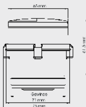
Measuring Capsule WMx10.D
